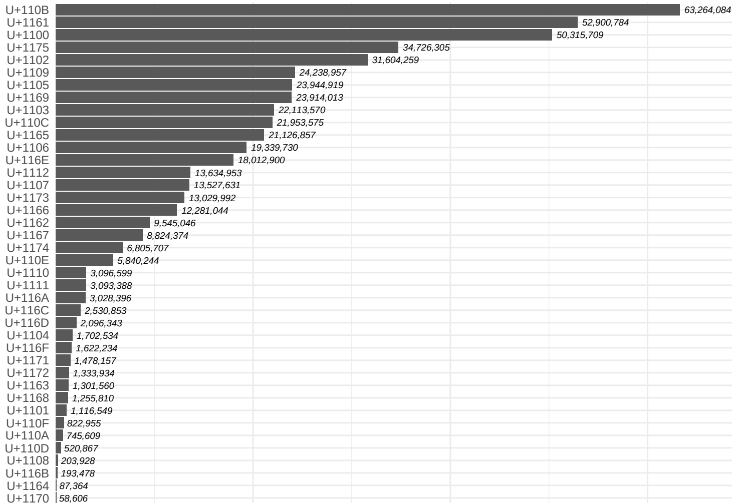
Total Instances of Jamo Unicode (Weighted by Word Frequencies)
